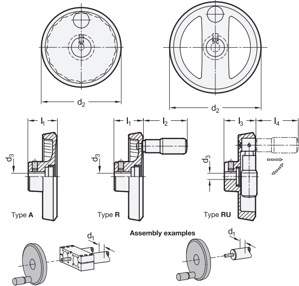
Disk handwheel
